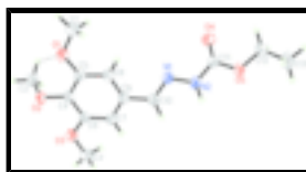
Fig. 1. The molecular structure of (I), showing 40% probability displacement ellipsoids for the non-hydrogen atoms. The C—H···O interaction is shown as a dashed line.
